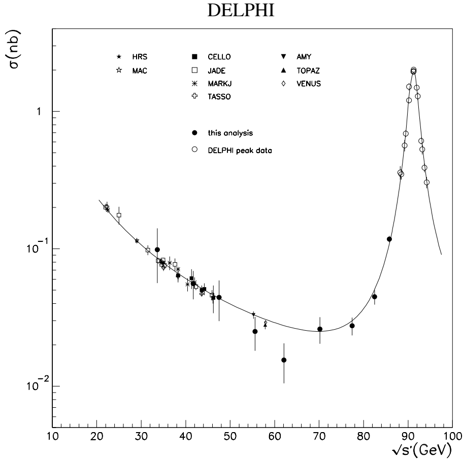
Fig. 16. Cross-sections in the Improved Born Approximation for \mu^+\mu^- as measured in the analysis of DELPHI data from 1992 to 1995 ( black circles ), at the Z^0 peak ( open circles ), and at PEP, PETRA and TRISTAN. The curve shows the SM prediction
