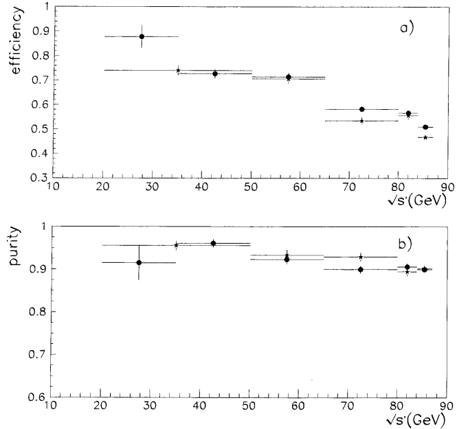
Fig. 14. a Efficiency for the selection of ISR events and b purity of the ISR sample with regard to FSR events, based on simulated radiative muon events, for the 1991-1994 data [27] (black dots) and for the data taken in 1995 (stars)
