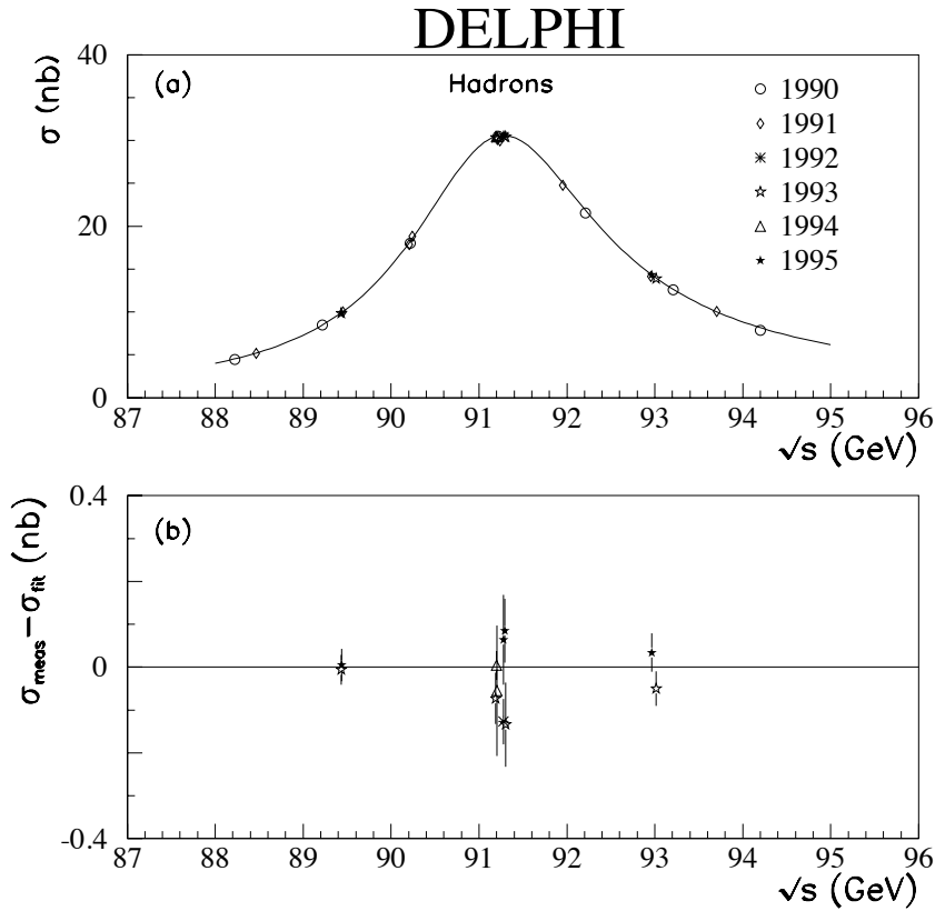
Fig. 18. Hadronic cross-sections from 1990, 1991, 1992, 1993, 1994 and 1995 data. The uncertainties shown are statistical only. In a the data are shown together with a curve representing the result of the 5-parameter fit described in Sect. 10. Plot b shows the difference of the measurements from the best fit values; for clarity only the data from 1992, 1993, 1994 and 1995 are shown
