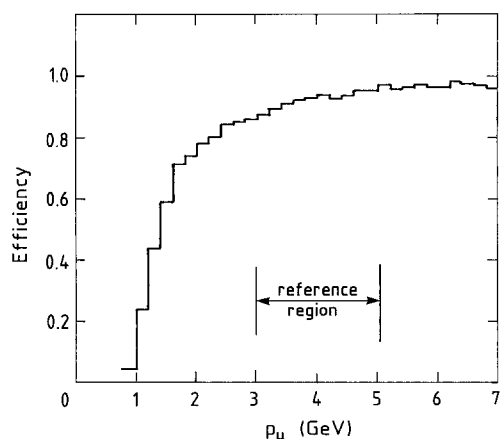
Fig. 11. Muon-finding efficiency
