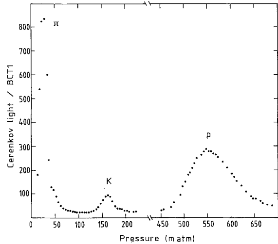
Fig. 14. Typical Cherenkov pressure curve in the neutrino beam
