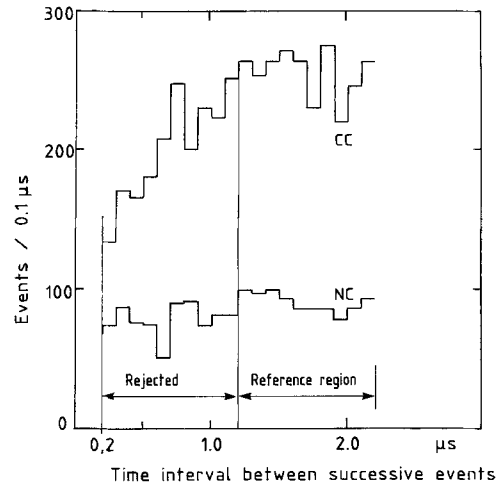
Fig. 4. Rejection of 'double events'
