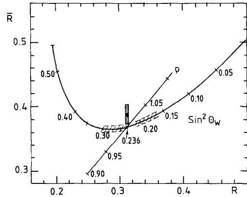
Fig. 15. Quark-model prediction for R^\nu and R^\nu as a function of \sin^2 \theta_W and \rho
